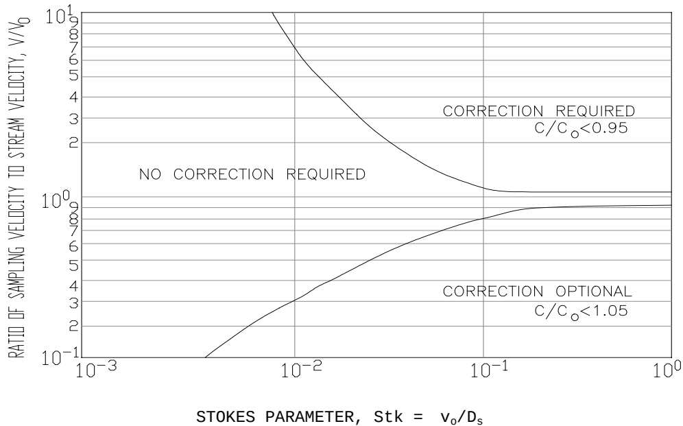
Figure C.3. Contours of sampling bias, C/C_0 = 0.95, 1.05
