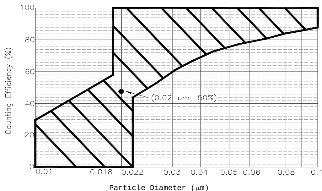
Figure D1. Envelope of acceptability for the counting efficiency of a DPC used to verify the U descriptor.
